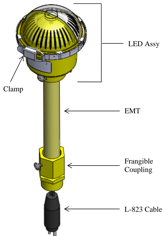
Figure 2-1 L-861 LED Light (Representative of all colors)
