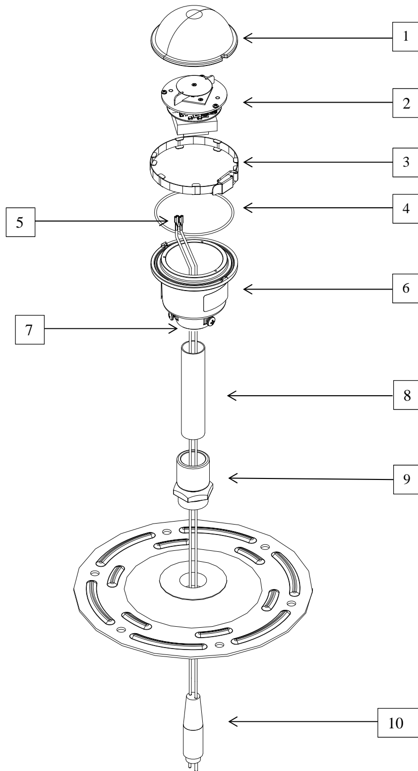
Figure 8-1 L-861 LED Light
